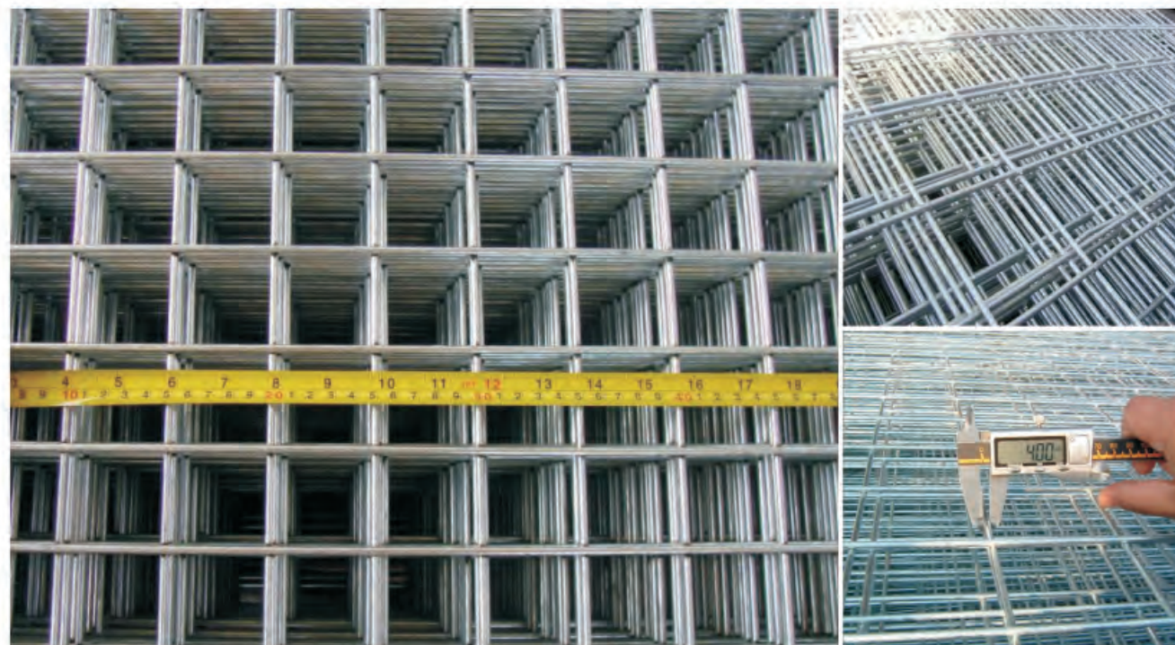
Welded mesh fabric reinforcement standard fabrics
